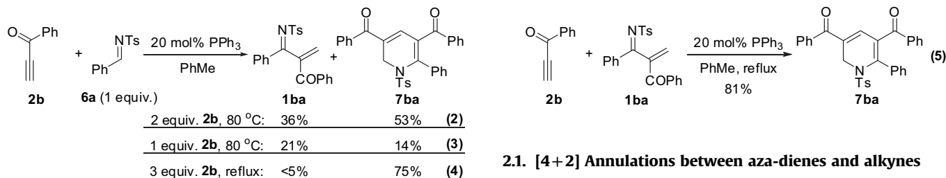
Scheme 2. The relationship between 1ba and 7ba .
