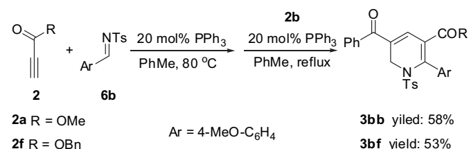
Scheme 3. Synthesis of 3bb and 3bf in one-pot way.
