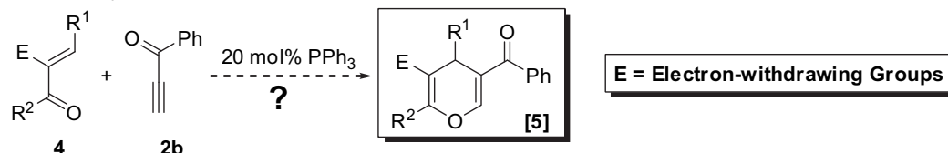
Scheme 1. Design plan for PPh 3 -catalyzed synthesis of dihydropyridines and dihydropyrans.
