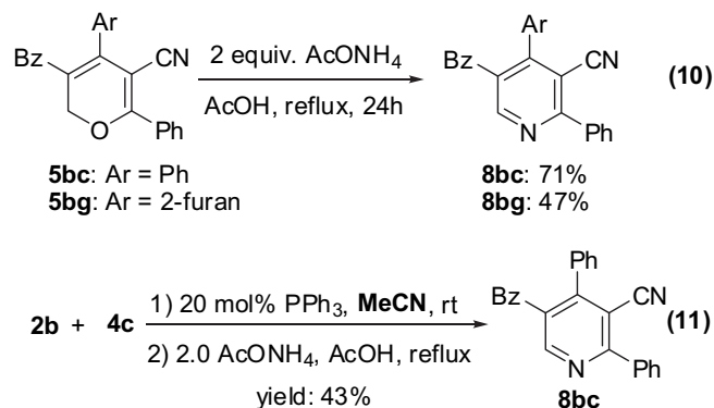
Scheme 6. Synthetic utility of 2 H -pyrans.
