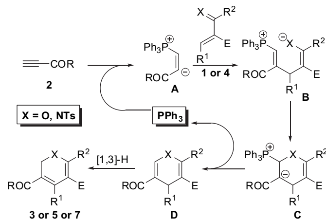
Scheme 4. Proposed mechanism for PPh 3 -catalyzed [4+2] annulations.
