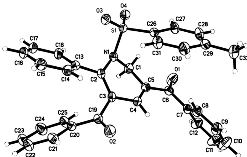
Figure 1. X-ray crystallography of 7ba . Ellipsoids at 30% probability.
