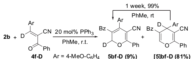
Scheme 5. Deuterium labeling studies.
